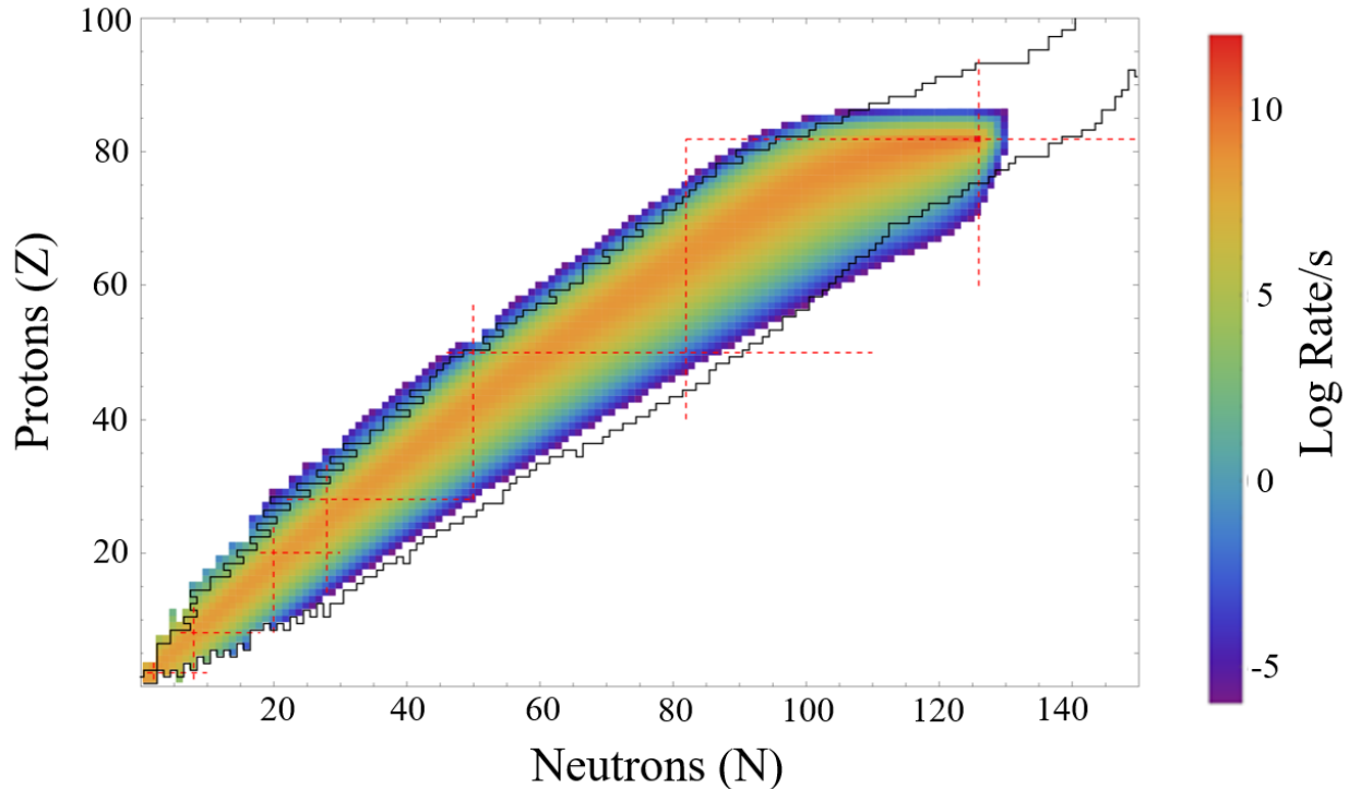
Figure 1.4: The production rate for each fragment of 212 MeV/u ^{208}\text{Pb} at 400 kW on a carbon target is shown. The EPAX3 parametrization was used for the cross sections, and the plot was generated in LISE++ version 16.0.3. Projectile fragments span the majority of the chart. The rate is shown in log scale and the highest intensity rates occur down and to the left of the primary beam.
