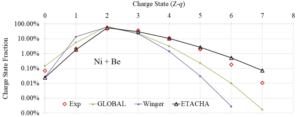
Figure 5.11: Charge state distribution of the primary beam, ^{198}\text{Pt}^{61+} , exiting the Ni + Be stripper setup. Experimental data is shown with red diamonds, ETACHA4.v3 [78] is shown in black triangles, GLOBAL [77] is shown in green, and Winger [90] is shown in purple.
