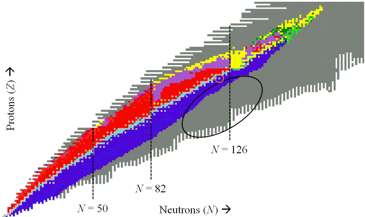
Figure 1.1: The Chart of Nuclides was generated in LISE ++ using the UNDEF1 mass model [6, 7]. Magic neutron numbers N = 126 , 82 , and 50 are denoted with a dashed black line. The region of interest for this work is denoted by the ellipse drawn with a solid black line. The orange circle slightly to the left of N = 126 denotes ^{198}\text{Pt} , the primary beam used in both fragmentation experiments presented in this thesis. The different colors on the chart indicate different types of radioactive decay. Red is \beta^+ decay, blue is \beta^- decay, and yellow is \alpha decay. Stable nuclei are shown in light grey, and undiscovered nuclei are shown in dark grey.
