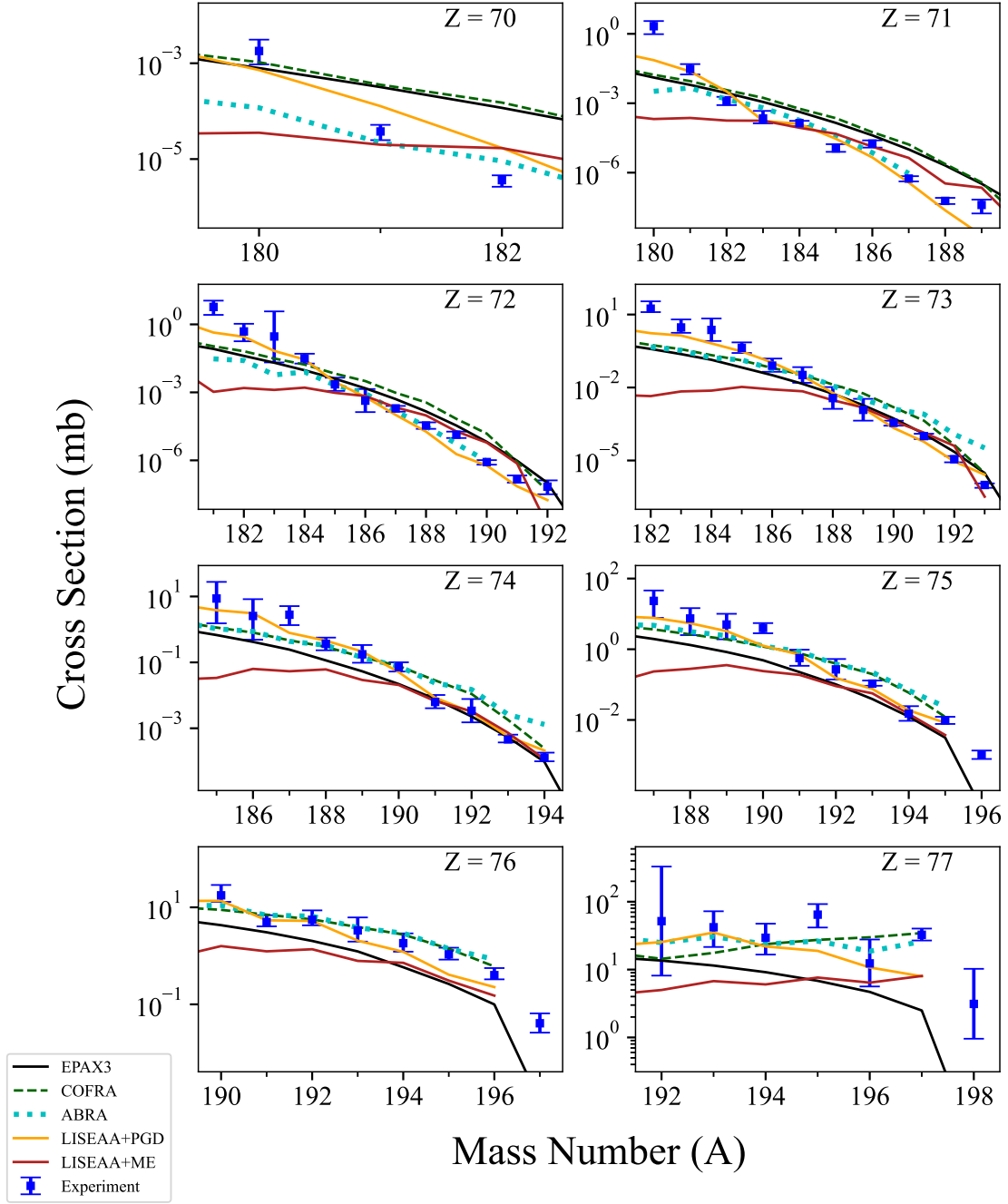
Figure 5.2: Experimental cross section measurements of 85 MeV/u ^{198}\text{Pt} + ^9\text{Be} are compared to five different models: EPAX3, COFRA, ABRA, LISEAA+PGD, and LISEAA+ME. The closest agreement occurs with LISEAA+PGD and ABRA models. A quantitative measure, calculated from an error-weighted average of residuals in log space is given in Table 5.1.
