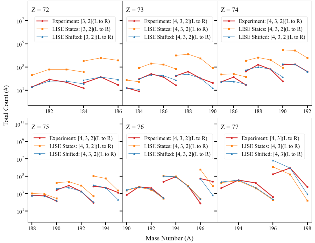
Figure 3.16: Yield curves for ions detected in data set D4a (red) are compared to LISE ++ predictions (orange). The LISE ++ curves are shifted (blue) to match the yield curves observed in experiment. A total of six elements are shown, hafnium through iridium.
