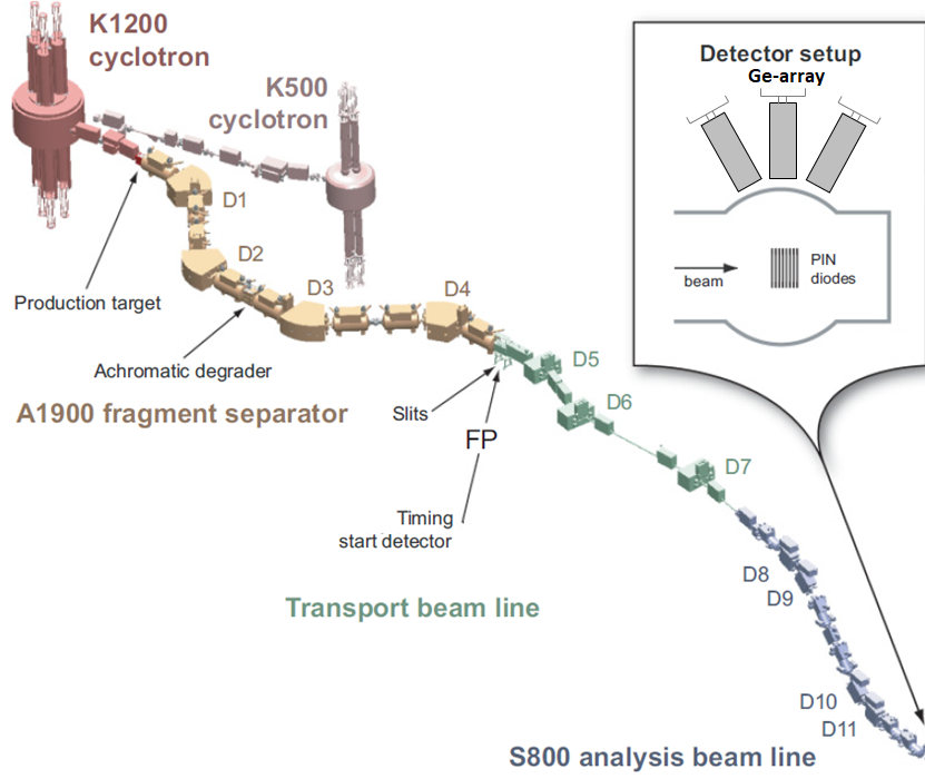
Figure 2.1: Sketch of the experimental setup used in the ^{198}\text{Pt} fragmentation experiment performed at NSCL, as presented in Haak et al. [23]. A ^{198}\text{Pt} beam was produced by the NSCL coupled cyclotrons and fragmented on a production target at the start of the A1900 fragment separator. Fragments were transported to the target location of the S800 spectrometer and stopped in a silicon telescope surrounded by GRETINA [59]. Image 1 (I1) of the A1900 was located between D2 and D3. I1 contained slits to define the momentum and an achromatic degrader (wedge). Image 2 (I2) was located at the focal plane of the A1900, labeled “FP”, and it contained another set of slits and a timing scintillator
