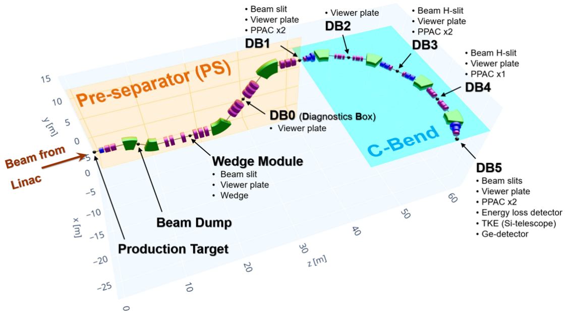
Figure 2.2: Sketch of the experimental setup used in fragmentation experiment performed at FRIB as presented in Tarasov et al. [67]. A ^{198}\text{Pt} beam was produced by the FRIB linear accelerator and fragmented on a production target at the start of the pre-separator. Fragments were transported to the diagnostic box 5 (DB5) where they were stopped in silicon to measure total kinetic energy and flight time.
