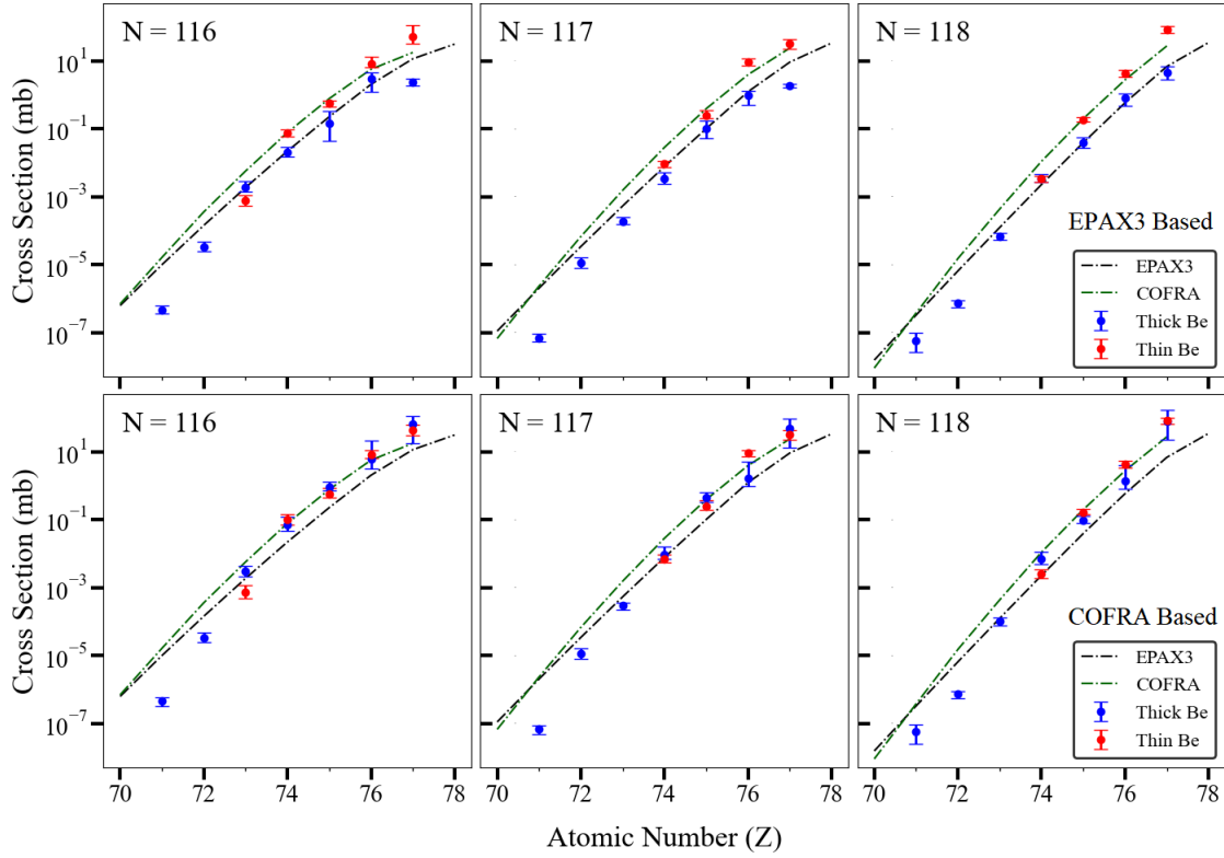
Figure 3.15: A comparison between final the cross section measurements produced from a COFRA based optimization (lower row) and EPAX3 based optimization (upper row). The result of both thin and thick target data sets are shown in red and blue respectively. As a reference, the cross sections predicted from EPAX3 and COFRA are shown by the the dashed black line and dashed green line, respectively. When using EPAX3 as a basis for optimization, the thin and thick target results disagree. The COFRA based optimization shows overlap within error for most data points.
