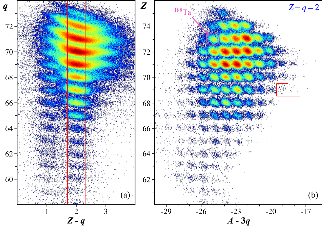
Figure 4.2: Two dimensional PID spectra of the fragments detected in the FRIB experiment, as presented in Tarasov et al. [67]. Spectrum (a) shows charge ( q ) vs charge state ( Z - q ), and spectrum (b) shows proton number ( Z ) vs mass ( A - 3q ). The separation of charge states is visible in (a) and a gate is drawn on the He-like charge state ( Z - q = 2 ). This gate is applied to spectrum shown in (b). The red line in the right spectrum indicated the limit of previously observed nuclides. ^{188}\text{Ta} is designated with a pink arrow for reference.
