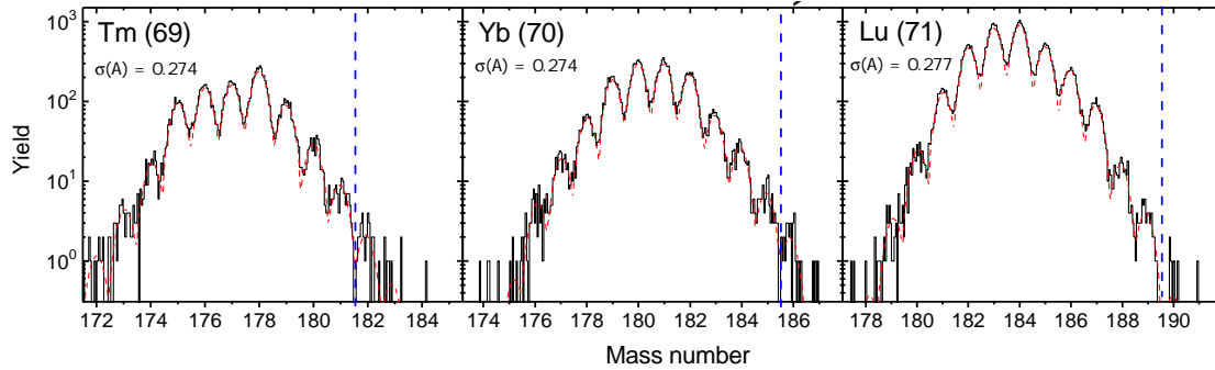
Figure 4.4: One dimensional mass spectra of fragments detected in the FRIB experiment, as presented in Tarasov et al. [67]. The black line is the experimental data represented in a histogram, the dashed red line is the series of Gaussian peaks fitted to the experimental data, and the blue dashed line is the previous boundary of discovery.
