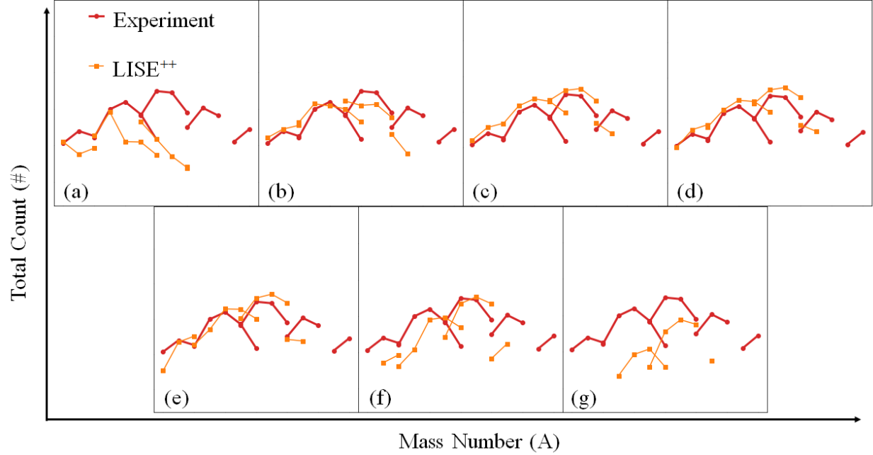
Figure 3.8: Experimental yields vs LISE ++ predictions plots used to infer the wedge parameters in run D4b (Ni target data). The isotopic chain for tungsten, Z = 74 and A = 184 to 196 , is shown for varying wedge thickness. A total of five different charge states, from Z - q = 4 to 0 , are shown from left to right respectively. Thicknesses 20.32 , 21.06 , 21.81 , 22.55 , 23.3 , 24.05 , and 24.8 \text{mg}/\text{cm}^2 are shown in (a) through (g) respectively. Based on this comparison we assume a wedge thickness of 22.55 \text{mg}/\text{cm}^2 .
