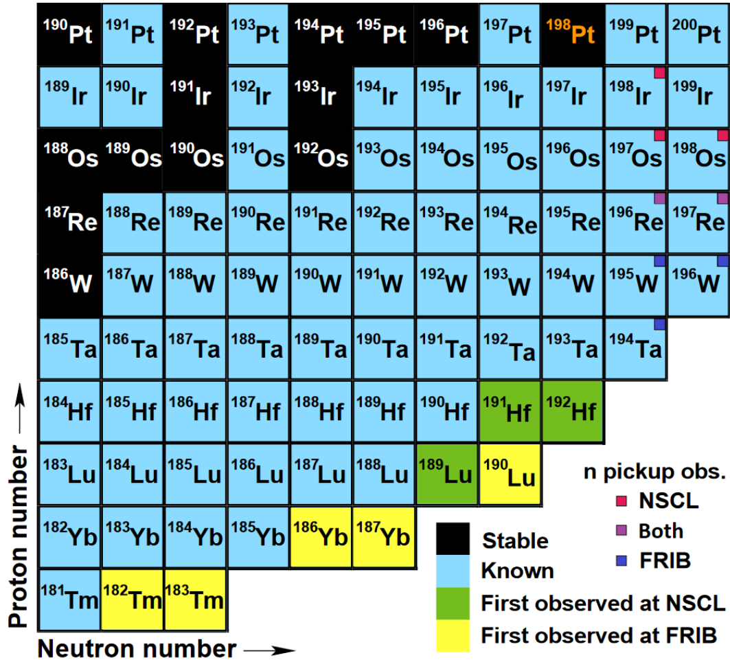
Figure 4.5: Chart of nuclides in the neutron-rich region “south” of ^{198}\text{Pt} , modified from Tarasov et al. [67]. New isotopes discovered at NSCL are shown in green, and new isotopes discovered at FRIB are shown in yellow. The small blue, red, and purple marks indicate pickup reactions observed in the FRIB experiment, the NSCL experiment, and both, respectively.
