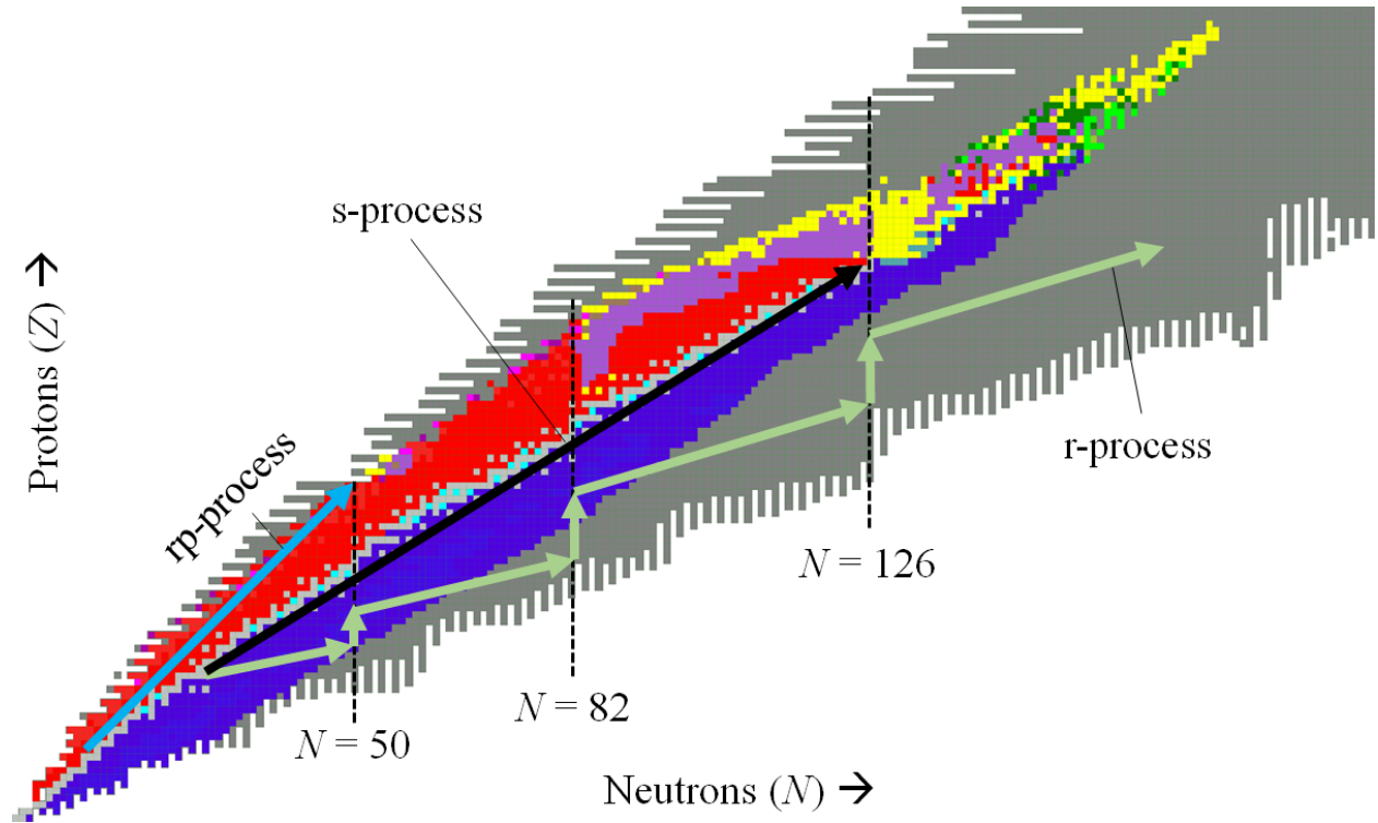
Figure 1.5: The Chart of Nuclides organized by nucleosynthesis processes [19]. The same color scheme for decay is used as in Figure 1.1. The rp-process, s-process, and r-process are represented by the blue, black, and green arrow, respectively.
