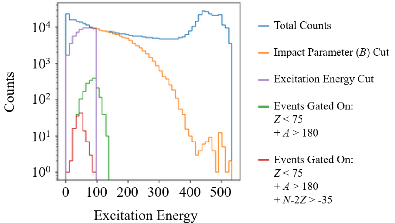
Figure 5.4: A histogram of pre-fragment excitation energies for events generated in the ABLA code. The impact of several gates are shown in the excitation energy spectra. An impact parameter ( B ) gate is shown in orange. Within the B gate, another excitation energy gate is shown in purple. The excitation energy of specific isotope regions are shown in red and green, as indicated in the key.
