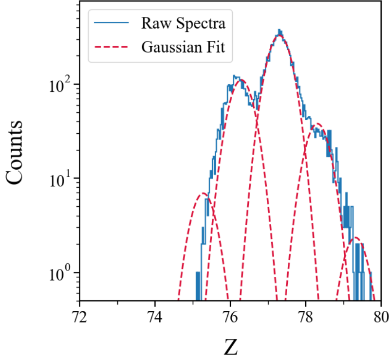
Figure 3.6: One dimensional fixed-width integer-spaced Gaussian peaks fitted to experimental data from Figure 3.5 (Ni target data). Raw spectra (blue) is the one dimensional Z histogram of data from the q = 74 AND A - 3q = 26 gate. Gaussian Fit (red) shows each individual Gaussian function fitted to their corresponding particle group.
