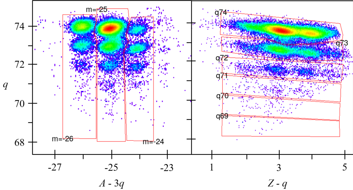
Figure 3.5: Visual example of gating procedure from Figure 3.4 (Ni target data). The data shown is from the Ni target data set D4a. The q vs mass ( A - 3q ) spectrum is shown with three mass gates on the left, and q vs charge state ( Z - q ) spectrum is shown with six charge gates on the right.
