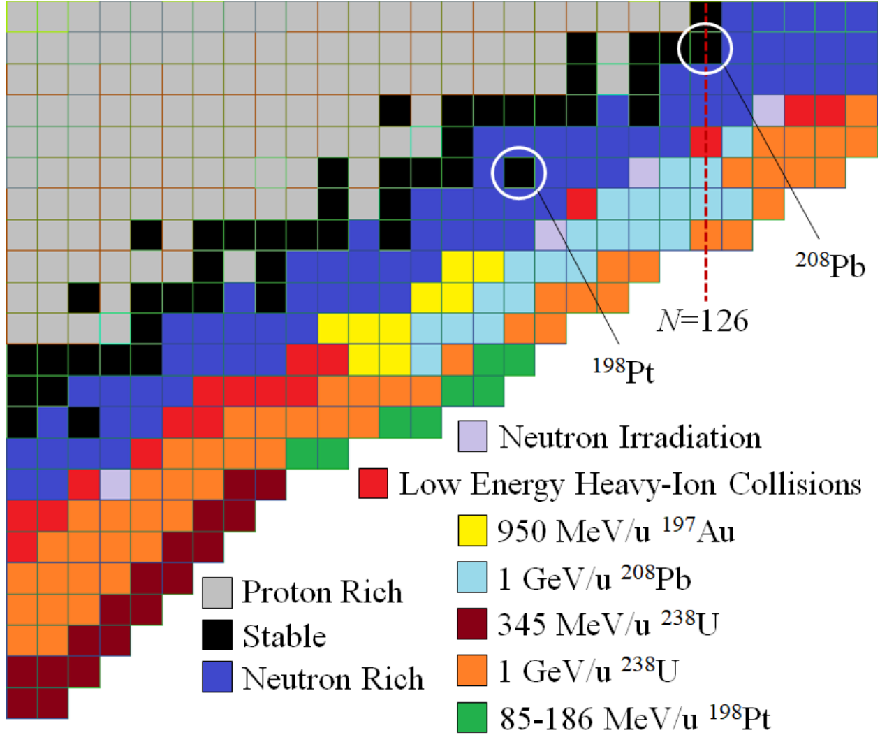
Figure 1.6: The neutron-rich region between 104 \leq N \leq 131 , organized by production methods that led to the first discovery of a given nuclide. Elements between Z = 61 promethium and Z = 83 bismuth are shown. The proton-rich side of the chart has been grayed out, the stable isotopes are shown in black, and neutron-rich isotopes discovered before 1980 are shown in blue. All low energy experiments are shown in red, neutron beam experiments are shown in light purple, and every other listed experiment was carried out using projectile fragmentation.
