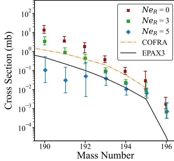
Figure 3.14: The cross sections of rhenium isotopes ( Z = 75 ) for three separate possibilities of Ne_R (0, 3, and 5), as presented in Haak et al. [23]. Each possibility shown here was calculated by an AEWa of charge states from the corresponding plot shown in Figure 3.13 (Be target data). The COFRA model, dashed orange line, has also been added in for reference.
