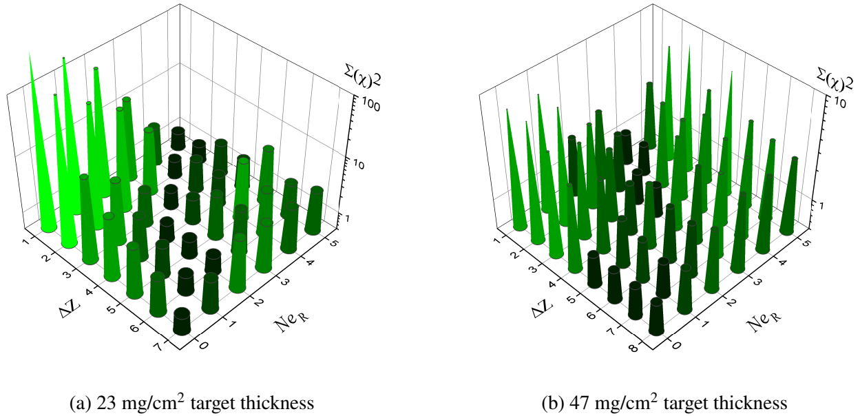
Figure 4.8: A summary of the most probable Ne_R values are presented for several values of abraded proton number ( \Delta Z ), derived from the analysis of experimental data, modified from Haak et al. [23]. Two different target thicknesses are shown, the thinner 23 mg/cm 2 target and the thicker 47 mg/cm 2 target. The vertical color axis represents a combination of three optimization considerations: agreement of cross section measurements between ions of the same nuclei, physically possible cross sections measurements, and the consistency of the production cross section for a specific element as a function of nucleon number.
