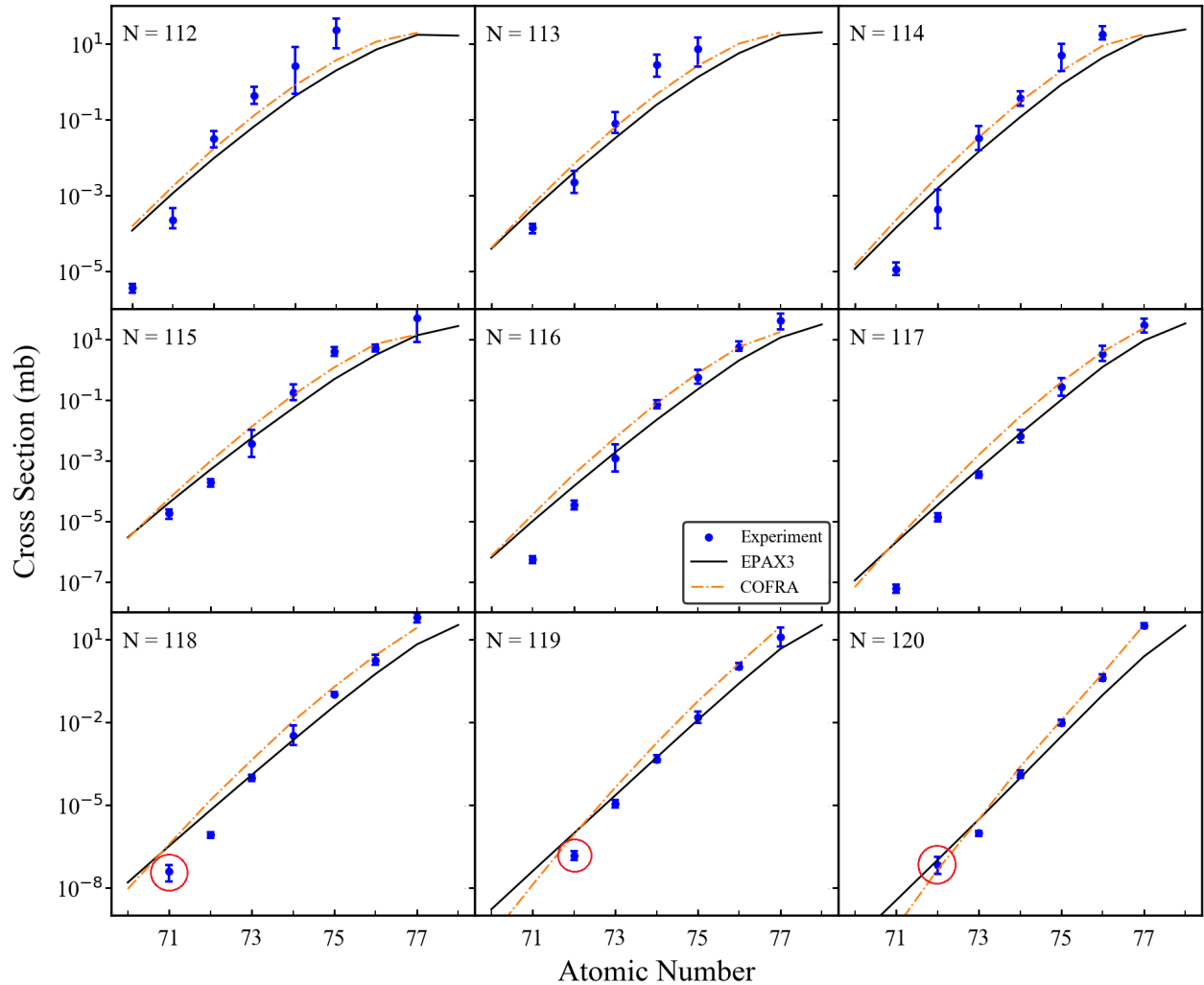
Figure 4.6: Cross section measurements of isotones ( N = 112 - 120 ) as a function of atomic number, as presented in Haak et al. [23]. These isotones were produced in the fragmentation reaction of ^{198}\text{Pt} (85 MeV/u) with ^9\text{Be} and are compared to EPAX3 and COFRA. New isotopes are denoted with red circles.
