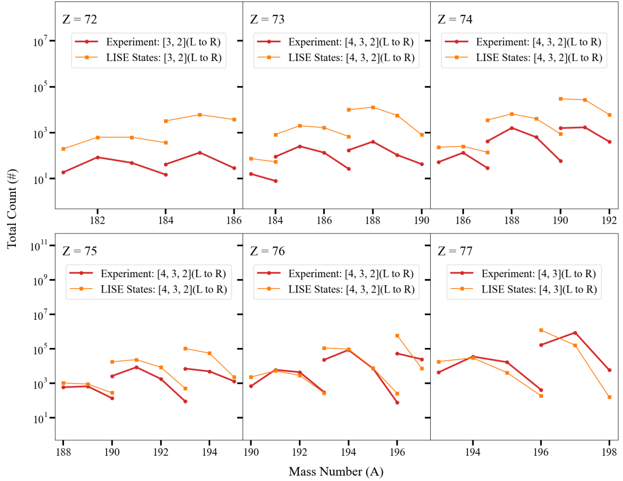
Figure 3.9: Optimized LISE ++ parameters matching experimental results from data set D4a (Ni target data). Counts of each ion are on the y-axis and mass number is on the x-axis. A total of six elements, with between two and three charge states per element, are shown. The charge states present in each plot are indicated by the legend and are listed in order from left to right (L to R). The experimental data is shown in red and the LISE ++ predictions are shown in orange.
