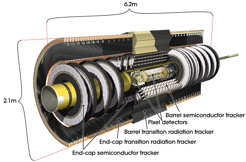
Figure 3.5: Cutaway illustration of the inner detector along with its subsystems [94].
