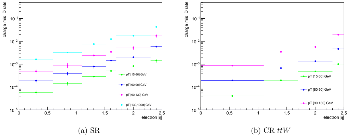
Figure 6.3: Charge flip rate calculated for SR and CR t\bar{t}W in bins of |\eta| and p_T .
