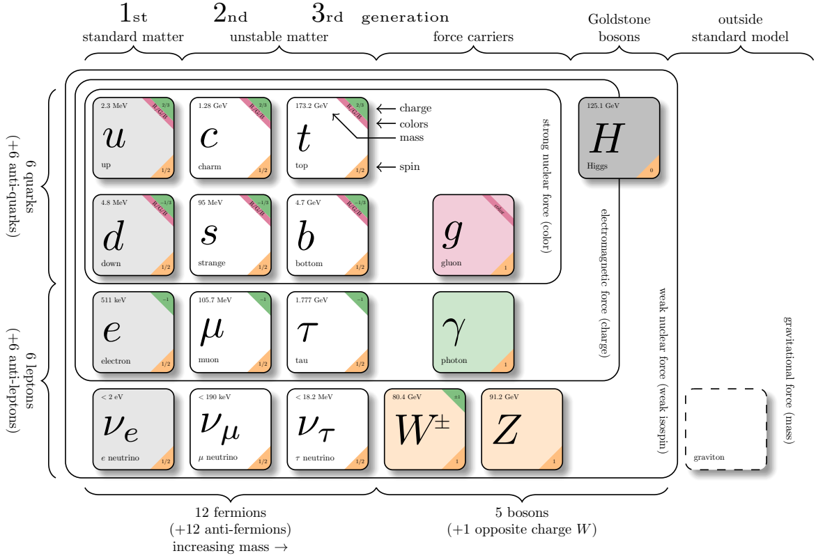
Figure 2.1: Particles within the SM and their properties [49].
