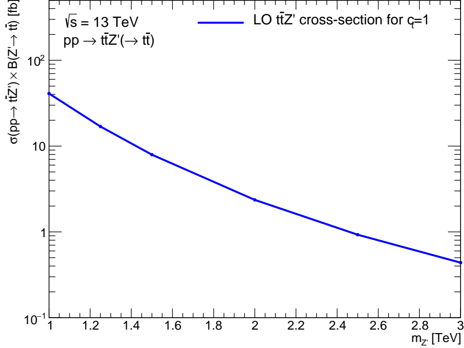
Figure 2.5: Theoretical t\bar{t}Z' production cross-section times Z' \rightarrow t\bar{t} branching ratio as a function of the Z' mass at LO in QCD coupling to top with c_t = 1 under a simplified top-philic model [45, 74, 77].
