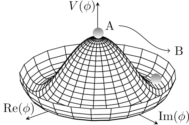
Figure 2.3: Illustration of a common representation of the Higgs potential [63]. Before SSB, the ground state \phi(0) is located at A which is symmetric with respect to the potential. A perturbation to this state fixes the ground state energy |\phi(0)|^2 to a particular value at B, "spontaneously" breaking the symmetry and degeneracy in |\phi(0)|^2 .
