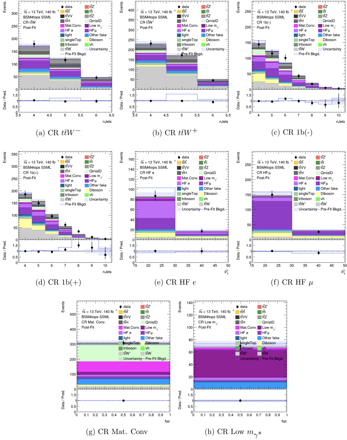
Figure 8.1: Comparison between data and post-fit prediction for the discriminant observable in each CR. Distributions shown are obtained from the fit using the t\bar{t}Z' signal sample with m_{Z'} = 2 TeV. The lower panel shows the ratio between data and post-fit predictions. The shaded band represents the total uncertainty on the fit. The dashed line represents the pre-fit distribution.
