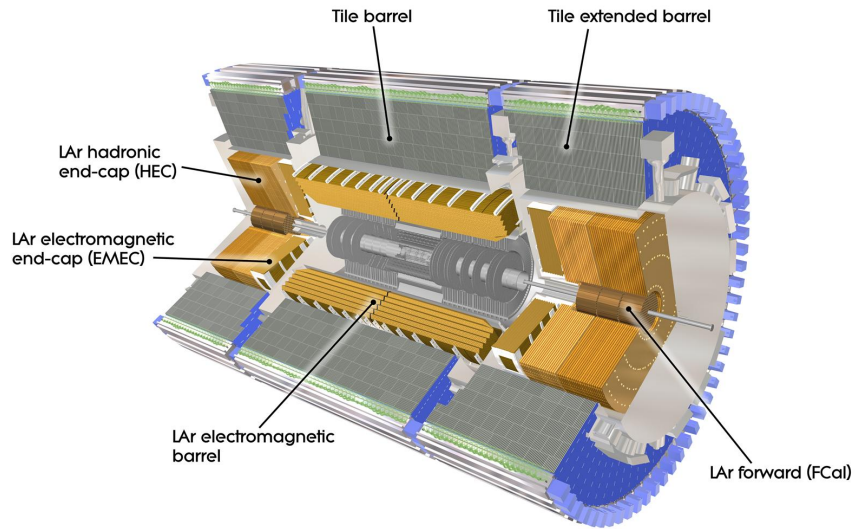
Figure 3.6: Cutaway illustration of the calorimeter system including the EM, hadronic and LAr forward calorimeters [95].
