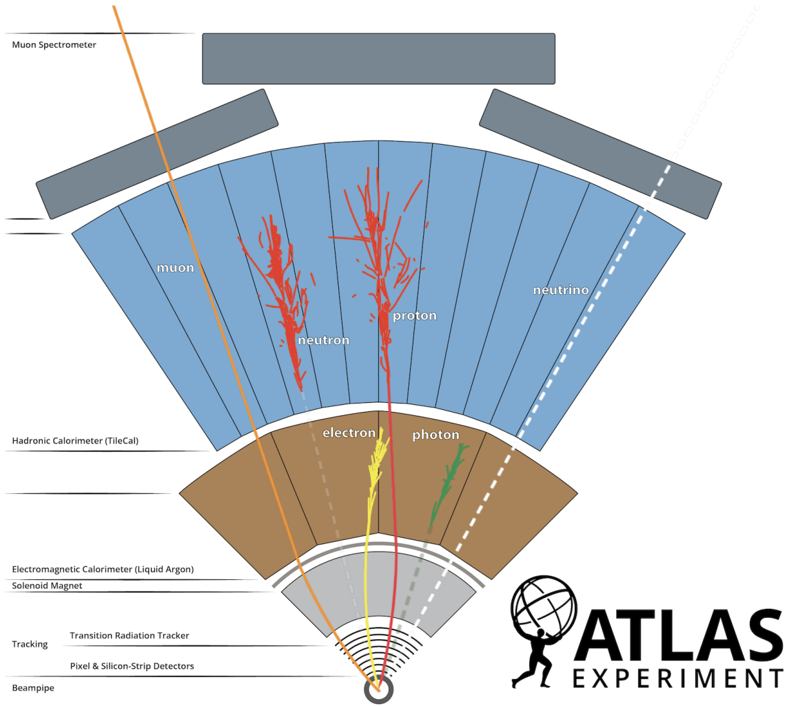
Figure 3.4: A cross section slice of the ATLAS detector showing different subsystems along with visualization of different types of particles traveling through the detector [93].
