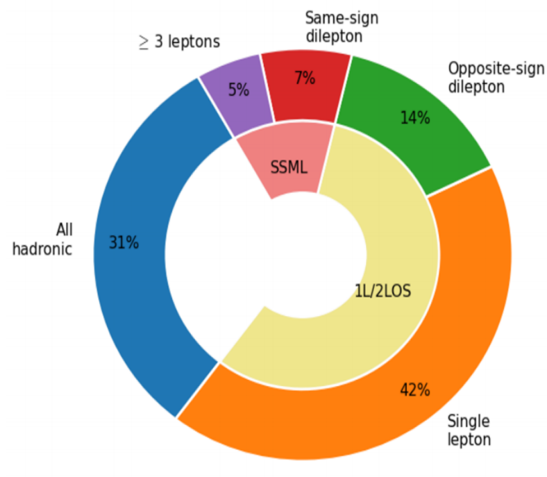
Figure 2.6: Branching ratios for t\bar{t}t\bar{t} decay [78]. The same-sign dilepton and multilepton channels together forms the SSML channel.
