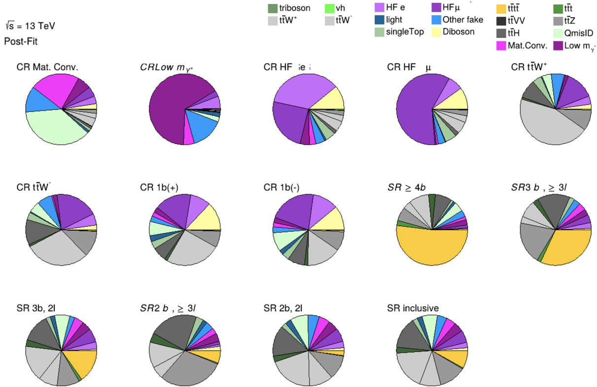
Figure 6.1: Post-fit background composition in each analysis region and sub-region. The fit was performed using ideal pseudo-datasets (Asimov data) in the SR.
