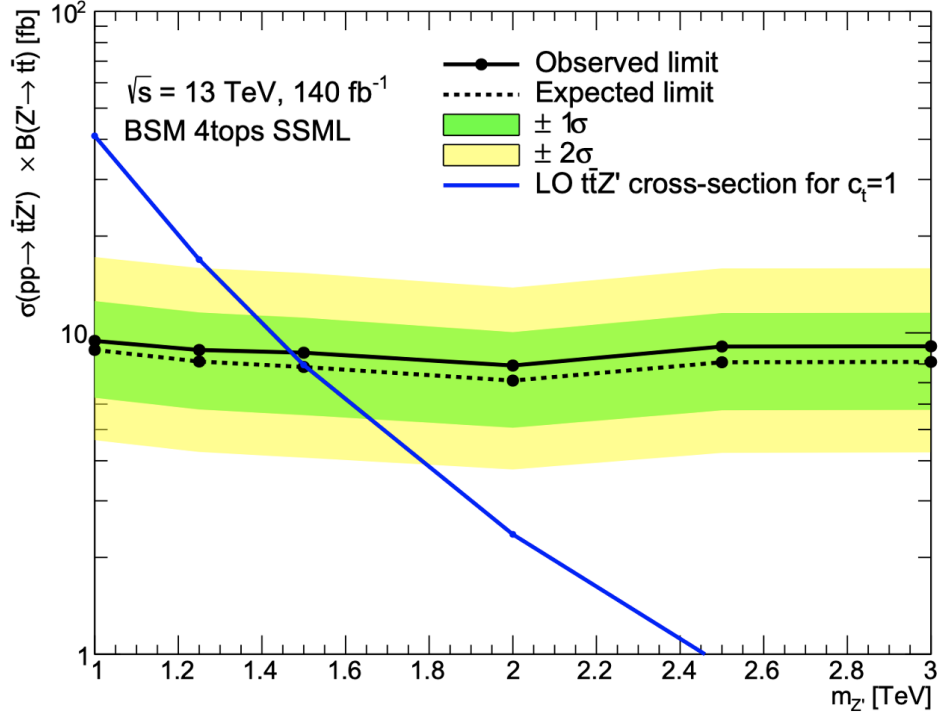
Figure 8.2: Observed (solid line) and expected (dotted line) upper limits as a function of the Z' mass at 95% CL on the cross-section of pp \rightarrow t\bar{t}Z' production times the Z' \rightarrow t\bar{t} branching ratio. The region above the observed limit is excluded. The solid blue line represents the theoretical signal cross-section with c_t = 1 at LO in QCD [74]. The green and yellow bands represent the 68% ( \pm 1\sigma ) and 95% ( \pm 2\sigma ) confidence intervals for the expected upper limits.
