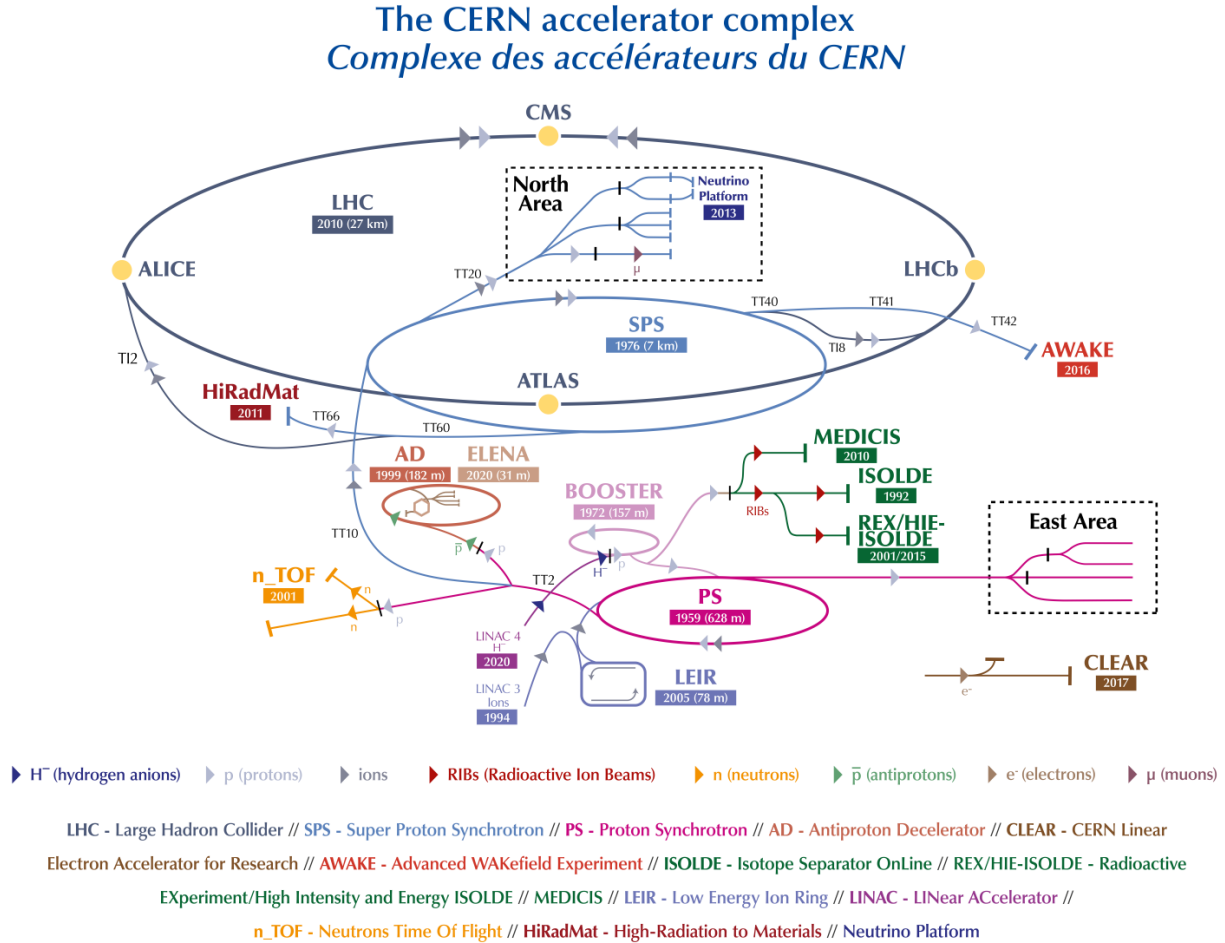
Figure 3.1: The full CERN accelerator complex as of 2022 [86].
