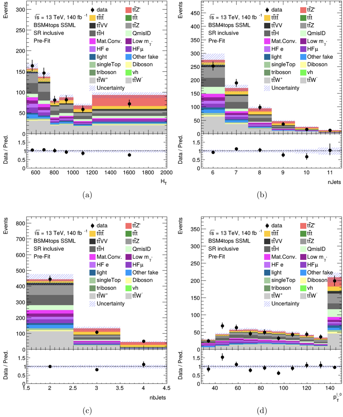
Figure 6.2: Pre-fit kinematic distributions and event compositions in the inclusive SR for (a) H_T i.e. scalar sum of p_T of all objects in the event, (b) jet multiplicity, (c) b -jet multiplicity, (d) leading lepton p_T . The shaded band represents the uncertainty in the total distribution. The first and last bins of each distribution contains underflow and overflow events respectively.
