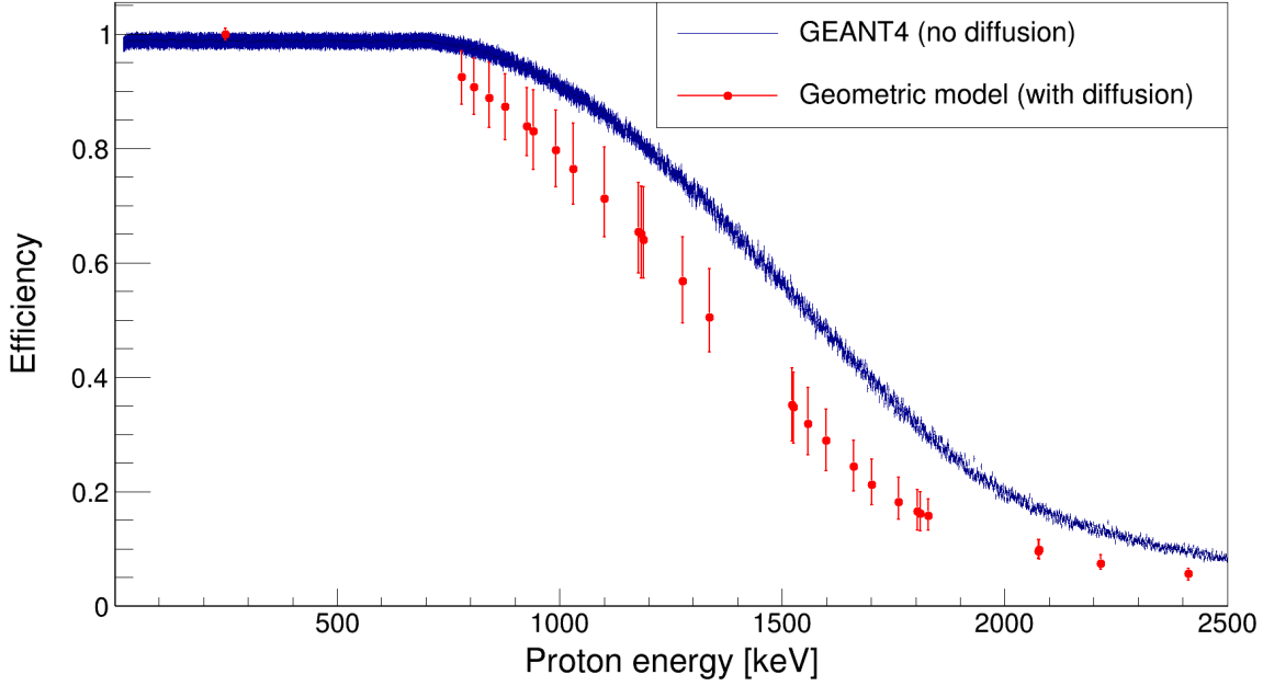
Figure 4.13: Efficiency to detect protons with GADGET as calculated by GEANT4 simulations assuming no electron diffusion (blue) and by the simplified, geometric model including the electron diffusion effect (red).
