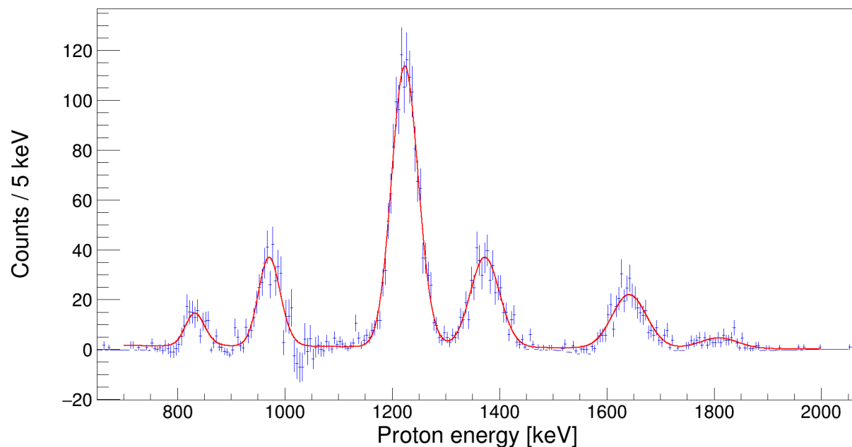
Figure 5.5: Background-subtracted energy spectrum for \beta -delayed protons in coincidence with 1454-keV \gamma decays to the ^{30}\text{P} ground state from the third excited state. This The six peaks were fit with EMG distributions, and the background is modeled as linear.
