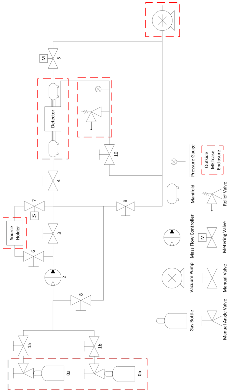
Figure 3.6: Schematic drawing of the custom-built gas handling system for GADGET.
