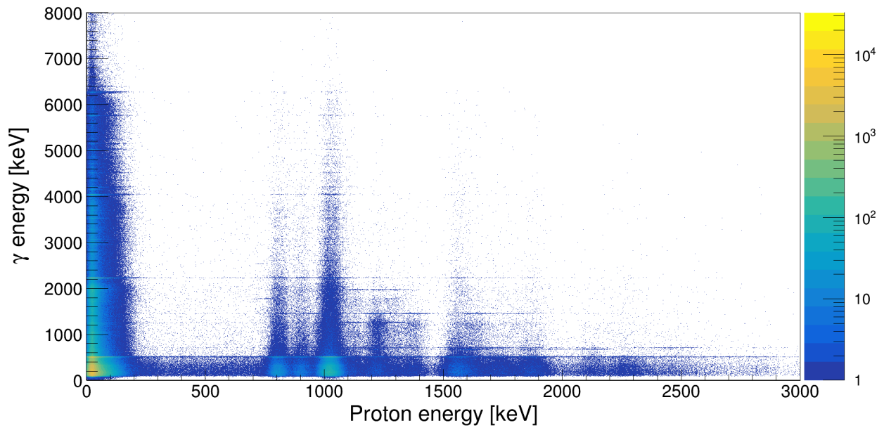
Figure 4.7: Two-dimensional coincidence matrix between \gamma rays detected in SeGA and charged-particle events in the Proton Detector.
