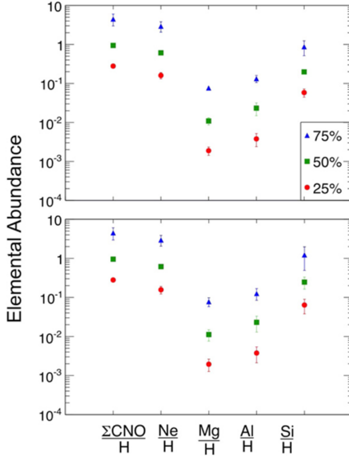
Figure 2.6: Elemental abundances, given in terms of their mass fraction relative to H, predicted in hydrodynamic nova model simulations. The three different marker types represent the mixing ratios between the underlying white dwarf material and the H-rich envelope. Top panel: Error bars only include variation due to changes in peak temperature. Bottom panel: Error bars include variation due to changes in peak temperature as well as uncertainties in thermonuclear reaction rates. Figure credit: [92].
