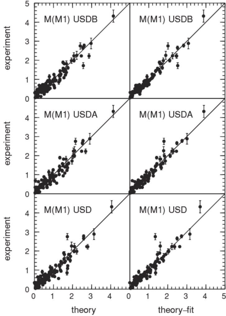
Figure 4.17: A comparison of experimental and theoretical values of the M1 matrix elements for magnetic dipole transitions. Figure credit: Ref. [152].
