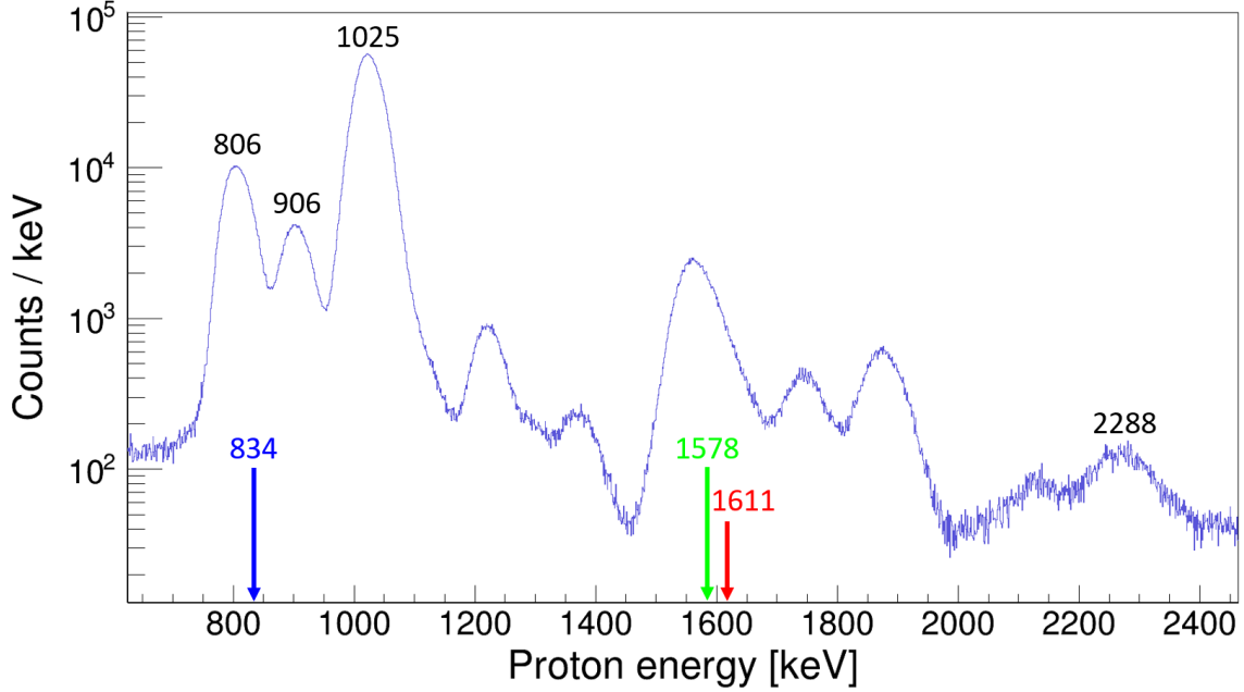
Figure 5.15: All proton peaks used in combined-pads energy calibration are color-coded by the ^{30}\text{P} levels their transitions populate directly. Visible singles peaks corresponding to ground state transitions (black) and weaker transitions to excited states (colored) are labeled by their center-of-mass decay energies in units of keV.
