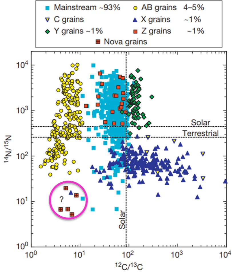
Figure 2.3: Isotopic ratios for plotted for C and N. Candidate nova grains are circled in magenta. Figure credit: Ref. [83].
