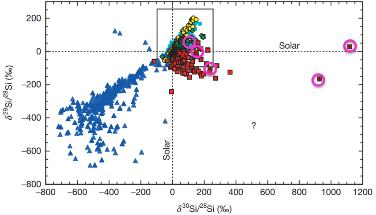
Figure 2.4: Isotopic ratios for plotted for Si. Candidate nova grains are circled in pink. Figure credit: Ref. [83].
