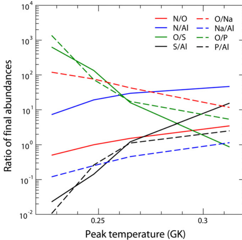
Figure 2.5: Ratios of elemental abundances, given in terms of their mass fractions, plotted as function of peak temperature achieved in hydrodynamic nova model simulations. Figure credit: Ref. [88].
