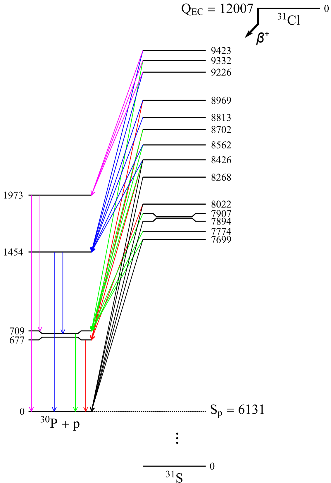
Figure 5.21: Possible decay scheme for ^{31}\text{Cl}(\beta p \gamma)^{30}\text{P} .
