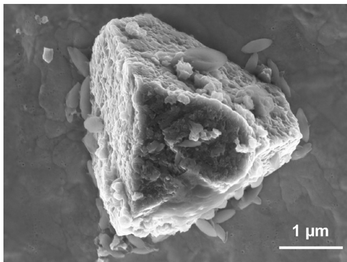
Figure 2.2: Electron microscope image of a SiC presolar. Photo credit: Max Planck Institute for Chemistry, J. Huth, A. Besmehn, and J. Kodolányi.
