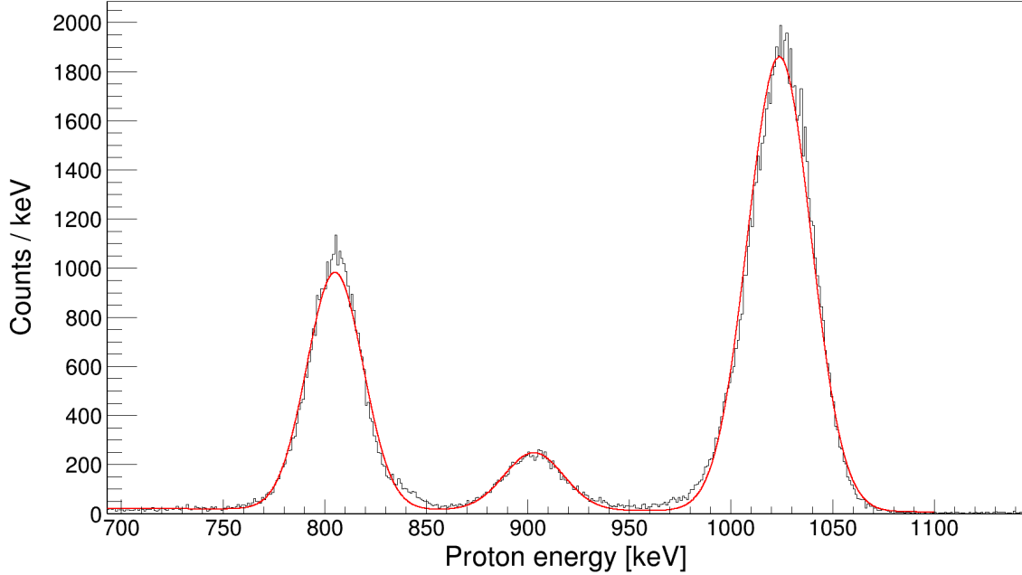
Figure 4.3: A \chi^2 -minimized fit of the calibration peaks as measured by the central pad of the Proton Detector. The three distributions were modeled as Gaussian and the background as linear.
