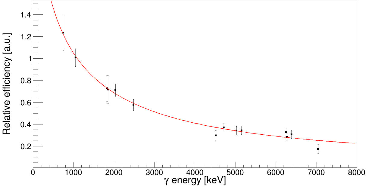
Figure 5.11: Relative efficiency to detect \gamma radiation in SeGA for events in coincidence with \beta -delayed proton decays.
