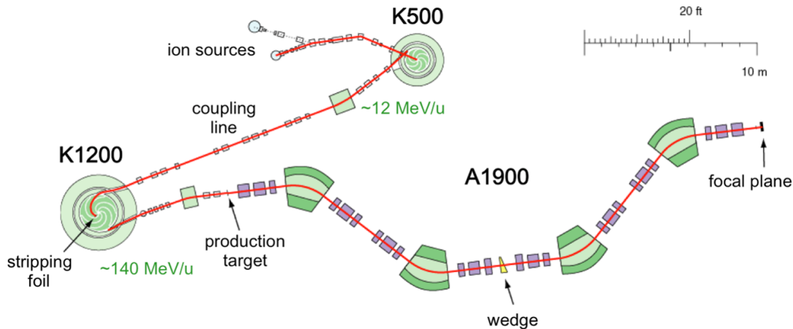
Figure 3.9: Diagram of the Coupled Cyclotron Facility and A1900 fragment separator at NSCL. Figure credit: Ref. [128].
