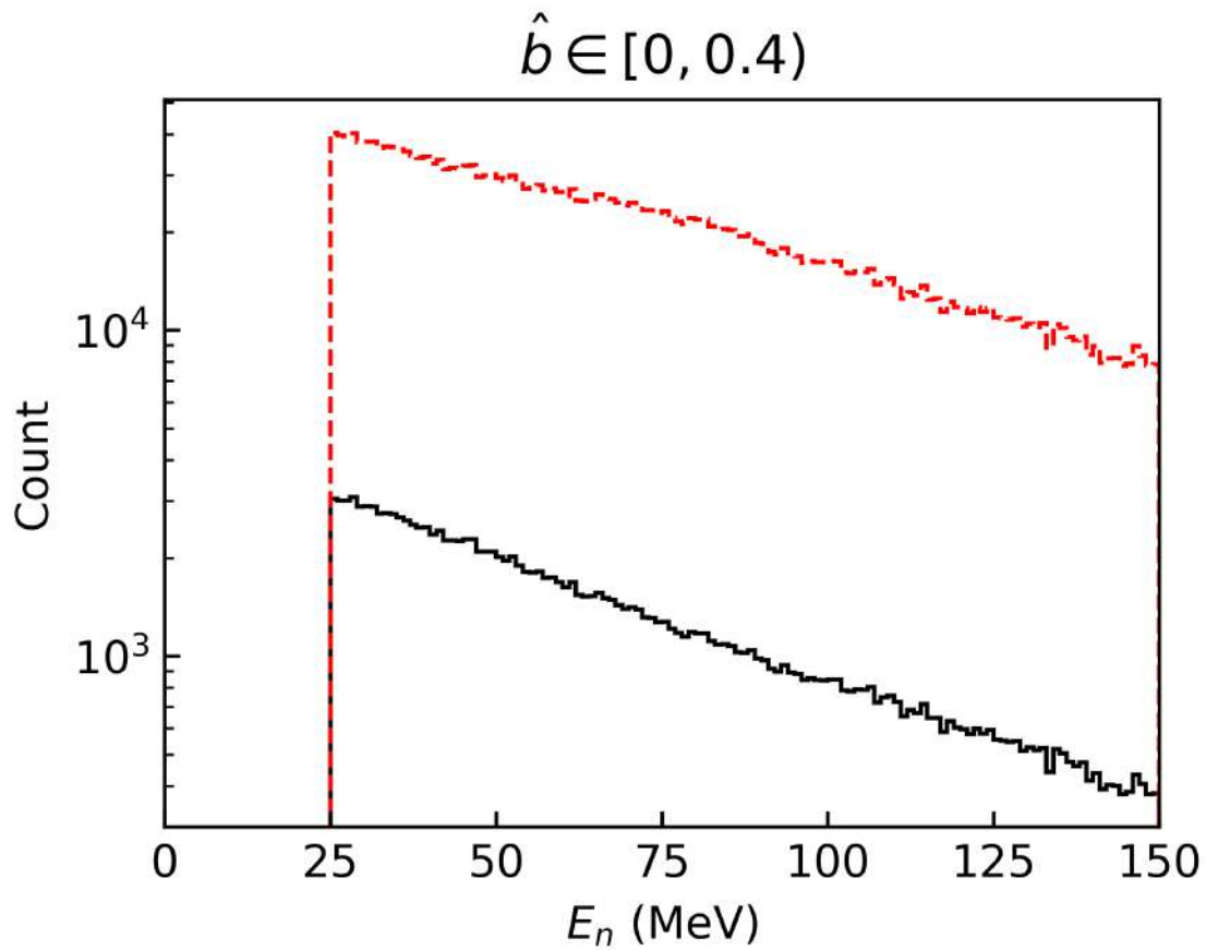
Figure 4.16: Neutron energy spectrum measured by the front LANA from ^{48}\text{Ca}+^{64}\text{Ni} at E/A = 140 \text{ MeV} reaction. The data come from a batch of continuous runs of around 18 hours. The Y-axis is counts per bin and the X-axis is neutron energy in MeV in lab frame. The black line represents the raw spectra and the red line shows the spectra after detection efficiency correction using the efficiency data from Fig. 4.15. All data shown here have a deduced impact parameter gate from [0, 0.4) .
