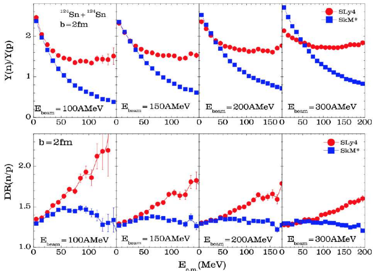
Figure 1.3: (top panels) Y(n)/Y(p) ratios as a function of kinetic energy for ^{124}\text{Sn}+^{124}\text{Sn} at b=2\text{fm} . (bottom panels) DR(n/p) ratios as a function of kinetic energy. From left to right, the beam energies are 100 MeV, 150 MeV, 200 MeV, 300 MeV per nucleon. Figure is adopted from Ref. [4].
