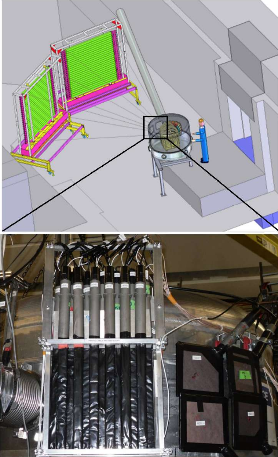
Figure 1.6: (top panel) Layout of the full experimental setup in the vault in previous experiment. (bottom panel) Image of the proton veto arrays (left) and paddles (right) attached to the outside of the reaction chamber. The vertical bars shadow the forward LANA, and the square paddles shadow the backward LANA. The forward LANA covers angles from 7^\circ to 29^\circ while the backward LANA covers angles from 34^\circ to 59^\circ . Pictures are adopted from Ref. [9].
