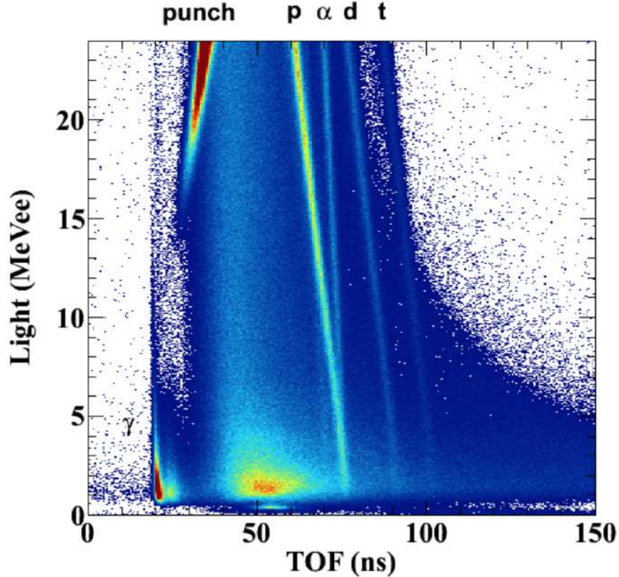
Figure 1.7: Neutron Wall light vs TOF, where TOF is the time of flight for the observed particle to travel to the neutron walls. The prompt \gamma ray peak, charged-particle punch-through, and charged particle stopping PID lines are marked. Picture is adopted from Ref. [9].
