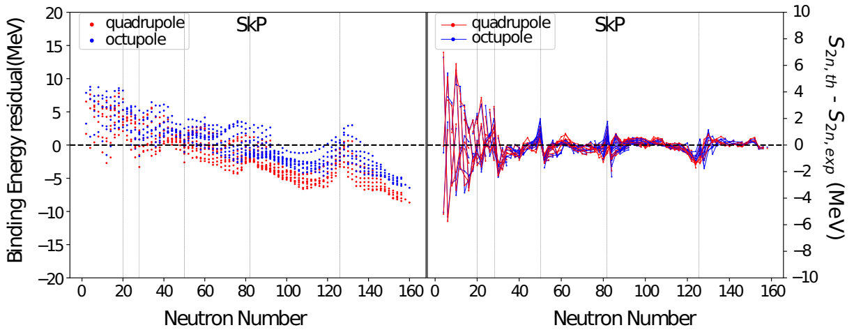
Figure 5.1: Left panel: Binding energy residuals of SEDF SkP (calculated w.r.t. experimental masses from the AME2016 mass evaluation [99, 159]). Results from octupole-deformed (blue dots) and quadrupole-deformed (red dots) survey calculations are shown. Right panel: Same as in left panel but for two-neutron separation energy S_{2n} . Note that the range on the energy axis is [-10, 10] MeV for S_{2n} compared to [-20, 20] MeV for BE, illustrating a significant reduction of systematic uncertainty in S_{2n} .
