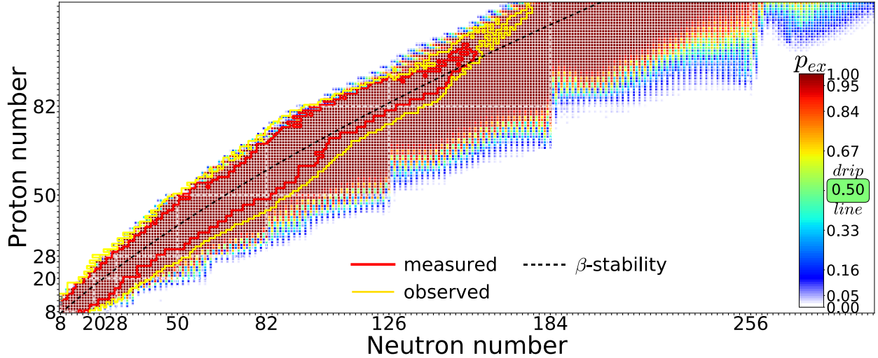
Figure 5.12: The quantified landscape of nuclear existence obtained in our BMA calculations. High-resolution of this figure can be found here . For every nucleus with Z, N \geq 8 and Z \leq 119 the probability of existence p_{\text{ex}} (5.27), i.e., the probability that the nucleus is bound with respect to proton and neutron decay, is marked. The domains of nuclei which have been experimentally observed and whose separation energies have been measured (and used for training) are indicated. To provide a realistic estimate of the discovery potential with modern radioactive ion-beam facilities, the isotopes within FRIB’s experimental reach are marked. The magic numbers are shown by straight (white) dashed lines, and the average line of \beta -stability defined as in Ref. [215] is marked by a (black) dashed line. In our estimates, we assumed the experimental limit for the confirmation of existence of an isotope to be 1 event/2.5 days. (Figure taken from Ref. [107])
