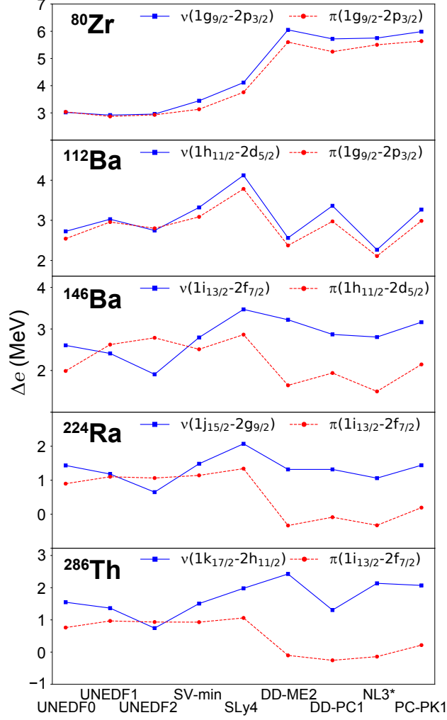
Figure 3.8: Single-particle energy splitting \Delta e between the unusual-parity intruder shell (\ell, j) and the normal-parity shell (\ell - 3, j - 3) for five nuclei representing different regions of octupole instability. The s.p. canonical states were obtained from spherical HFB/RHB calculations. The neutron (proton) splittings are indicated by the solid (dashed) lines. (Figure taken from Ref. [92])
