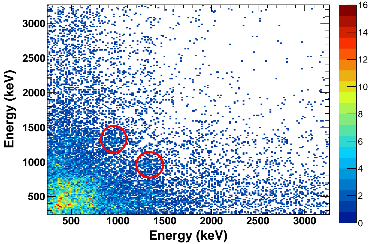
Figure 4.17: Doppler-corrected coincidence matrix for ^{44}\text{S} events with exactly two \gamma rays detected in CAESAR. Both the x and y axes have 16-keV wide bins. The matrix is filled symmetrically. The 1329-keV transition is in coincidence with the 949-keV transition.
