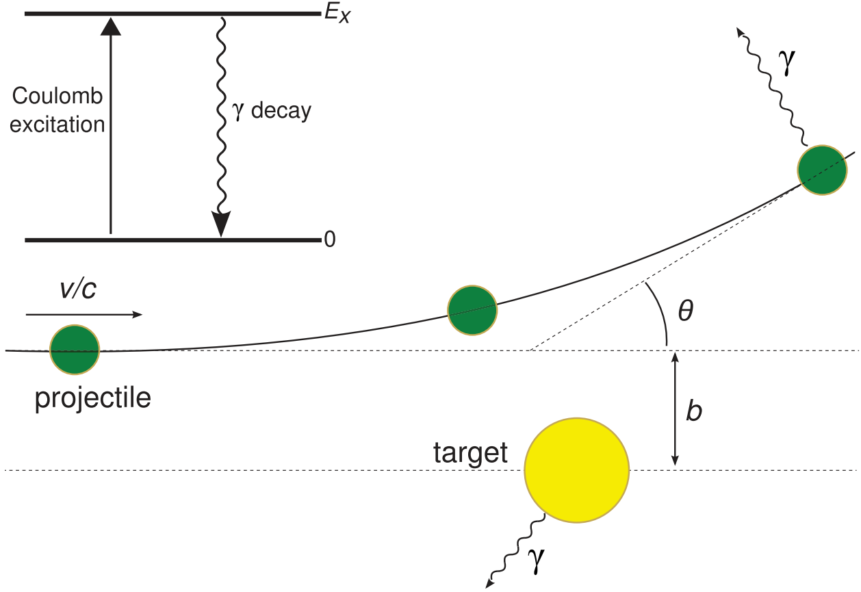
Figure 2.1: Schematic of intermediate-energy Coulomb excitation. The projectile (target) nucleus is inelastically excited in the Coulomb field of the target (projectile) nucleus. In analysis, a maximum center-of-mass scattering angle \theta (minimum impact parameter b ) is considered to ensure no nuclear contribution to the cross section. Figure adapted from [11].
