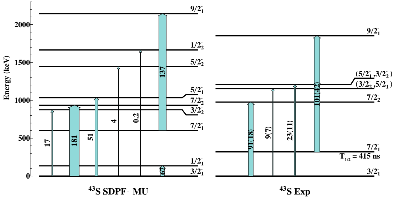
Figure 4.24: SDFP-MU predictions for B(E2) strengths in e^2\text{fm}^4 for low-lying levels in ^{43}\text{S} compared with experimental results. Arrow widths are proportional to transition strength.
