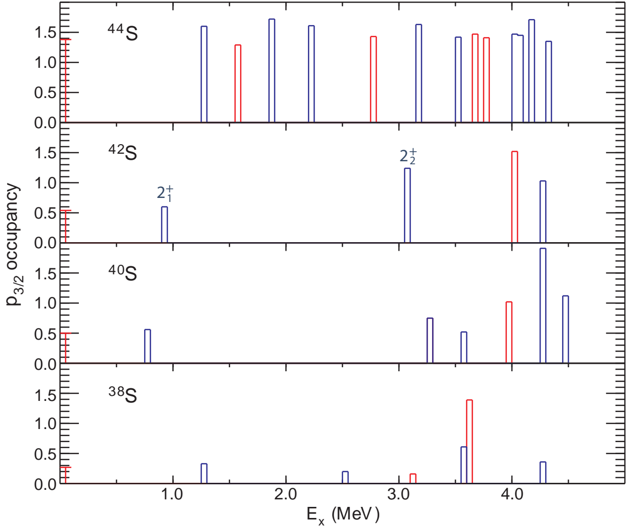
Figure 1.8: SDPF-MU neutron 1p_{3/2} occupancies for 0^+ (red) and 2^+ states (blue) below 4.5 MeV in ^{38,40,42,44}\text{S} . The increase in occupancy for the second 2^+ state in ^{42}\text{S} relative to ^{38}\text{S} explains the observed change in \gamma -decay pattern. Figure modified from [10].
