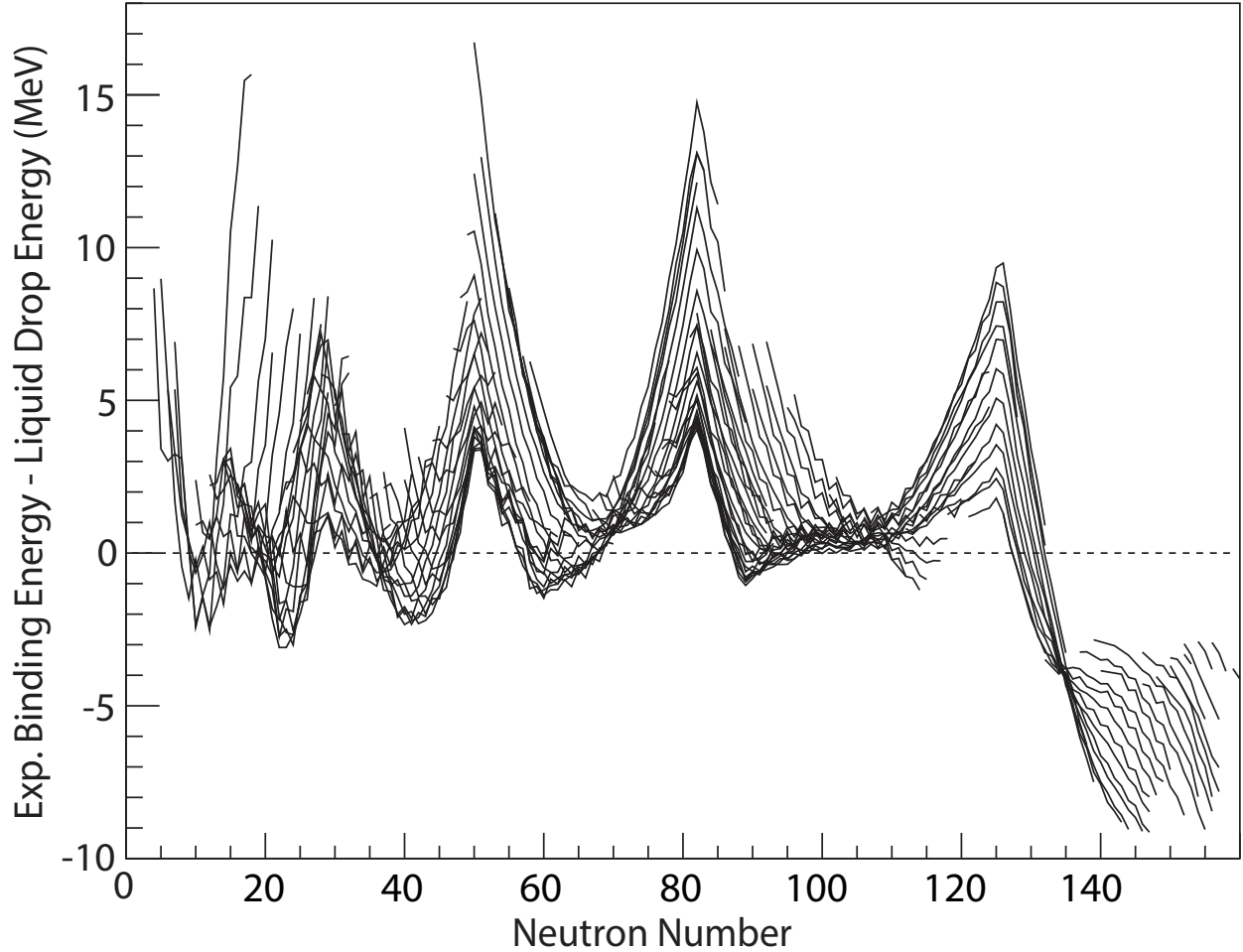
Figure 1.3: Differences between experimental binding energies and binding energies calculated using the liquid drop model for nuclei with Z \geq 8 as a function of neutron number. The peaks at N=28, 50, 82, and 126 indicate that nuclei have internal structure. Figure taken from [3] with data from [4].
