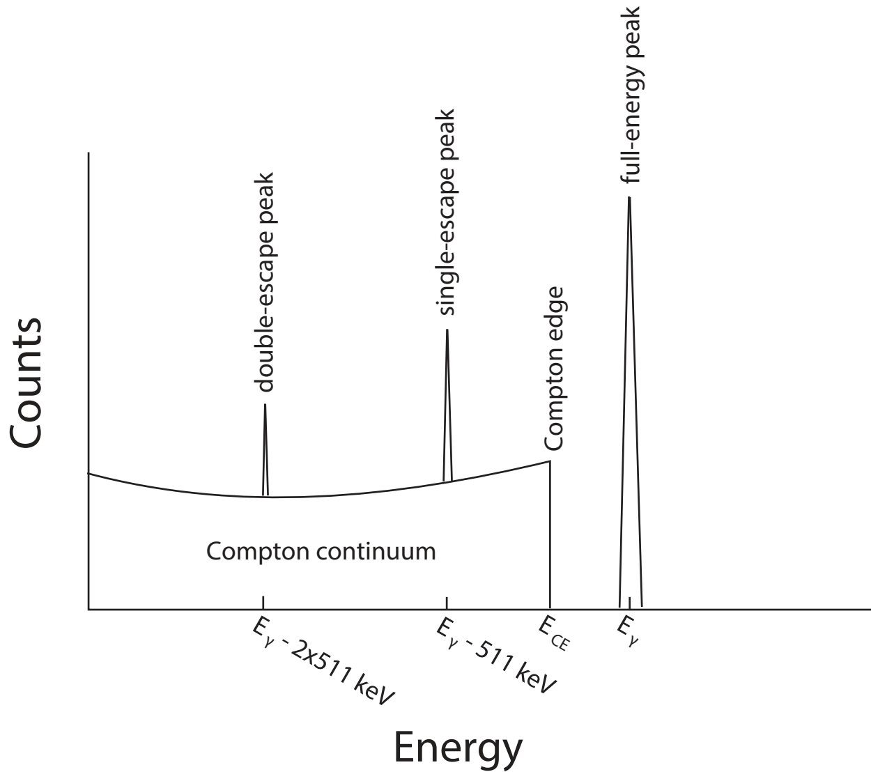
Figure 3.8: Illustration of the response of a \gamma -ray detector to many monoenergetic \gamma rays showing characteristic features including the full-energy peak, Compton edge, Compton continuum, and single and double-escape peaks. Figure taken from [11].
