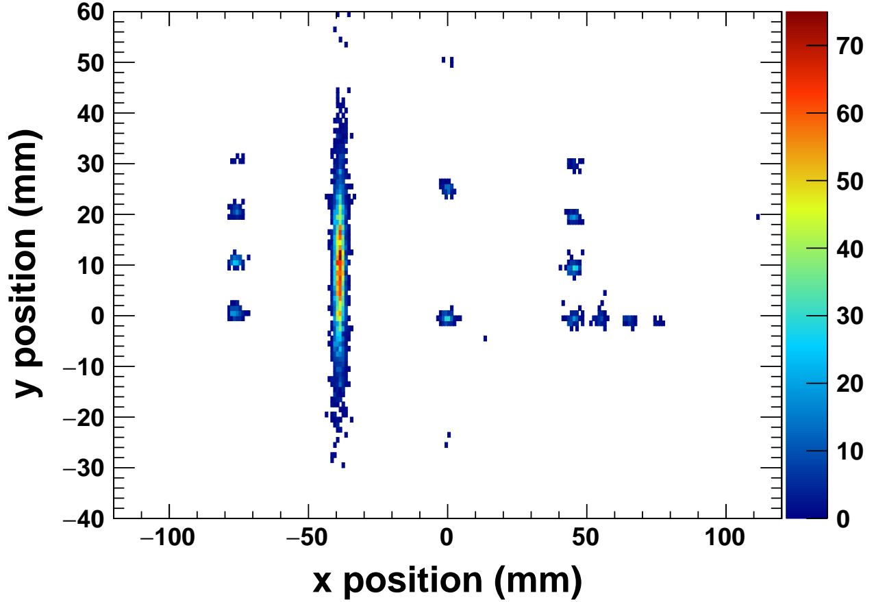
Figure 3.4: Typical calibrated mask run for CRDC1 (upstream) taken from the ^{38}\text{S} setting.
