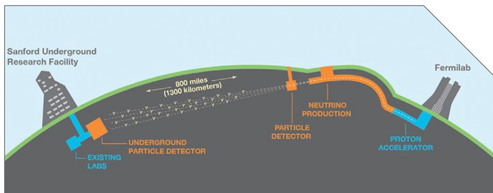
Schematic of the Long-Baseline Neutrino Facility.
