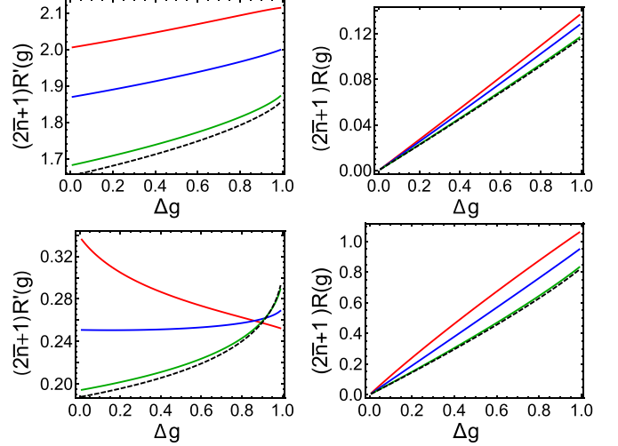
FIG. 15. The dependence of the functions R'(g) (left panels) and R(g) (right panels) on the RWA energy g for \delta\omega > 0 , \Delta g = (g - g_{\text{min}})/(g_s - g_{\text{min}}) . The scaled drive amplitude is f = 0.1 (upper panels) and f = 2 (lower panels). The red, blue, and green solid lines (top, middle, and bottom, for \Delta g < 0.8 ) refer to \bar{n} = 0, 0.1, 1 , respectively. The dashed black line refers to the classical limit in Eq. (28). For the chosen values of the driving amplitude there holds the locality condition, and thus the distribution can be found in the eikonal approximation, as can be seen from Fig. 6.
