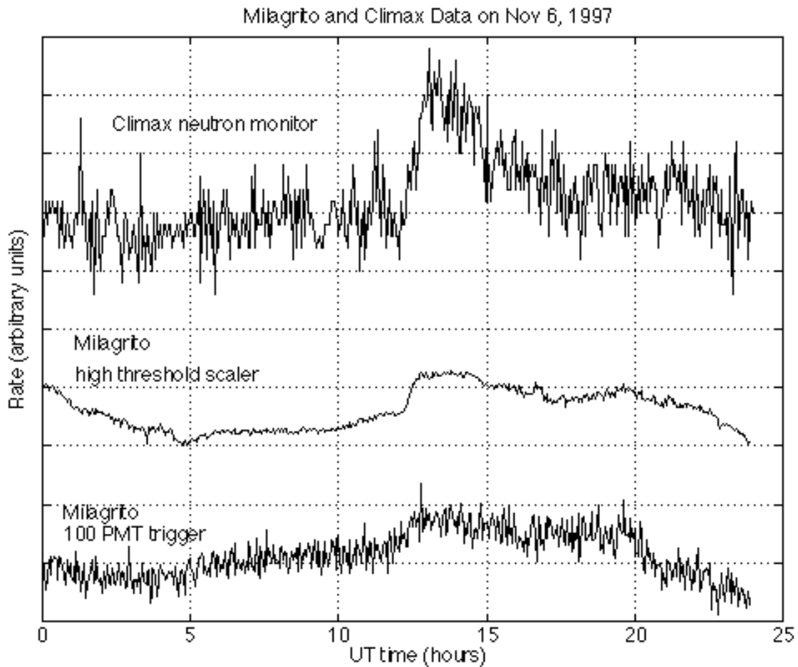
FIGURE 2. Milagrito registered a rate increase coincident with that of Climax during the GLE of Nov. 6, 1997. The y-axis units have been scaled and shifted for each plot to make comparison easier. (Climax data courtesy of C. Lopate, Univ. of Chicago)
