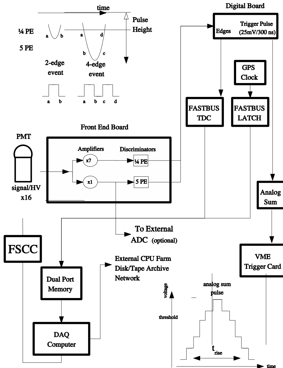
Figure 5.10: Schematic of the Milagro's electronics system. Source [35]
