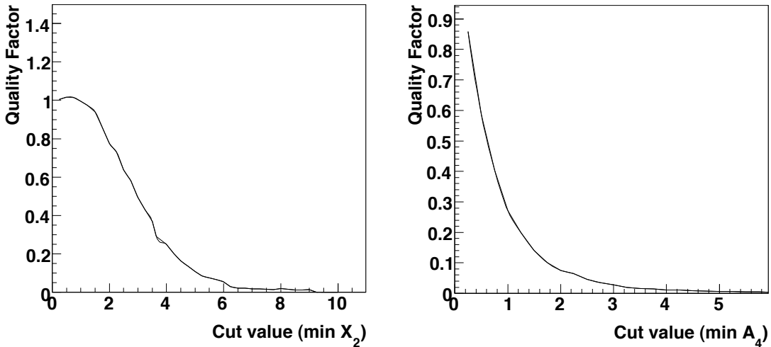
Figure 6.7: Effect of applying the standard gamma-hadron discrimination cuts to the signal from a source emitting on a power-law spectrum with index -2.00 from redshift 0.3 . The quantity plotted is the quality factor defined as Q = \frac{f_S}{\sqrt{f_B}} , where f_S and f_B are the fractions of signal and background that pass a specific cut. The quality factor shows the change in the statistical significance of a signal introduced by applying a cut. These plots are only valid for the longer durations, where the large statistics allow Gaussian probabilities to be used.
